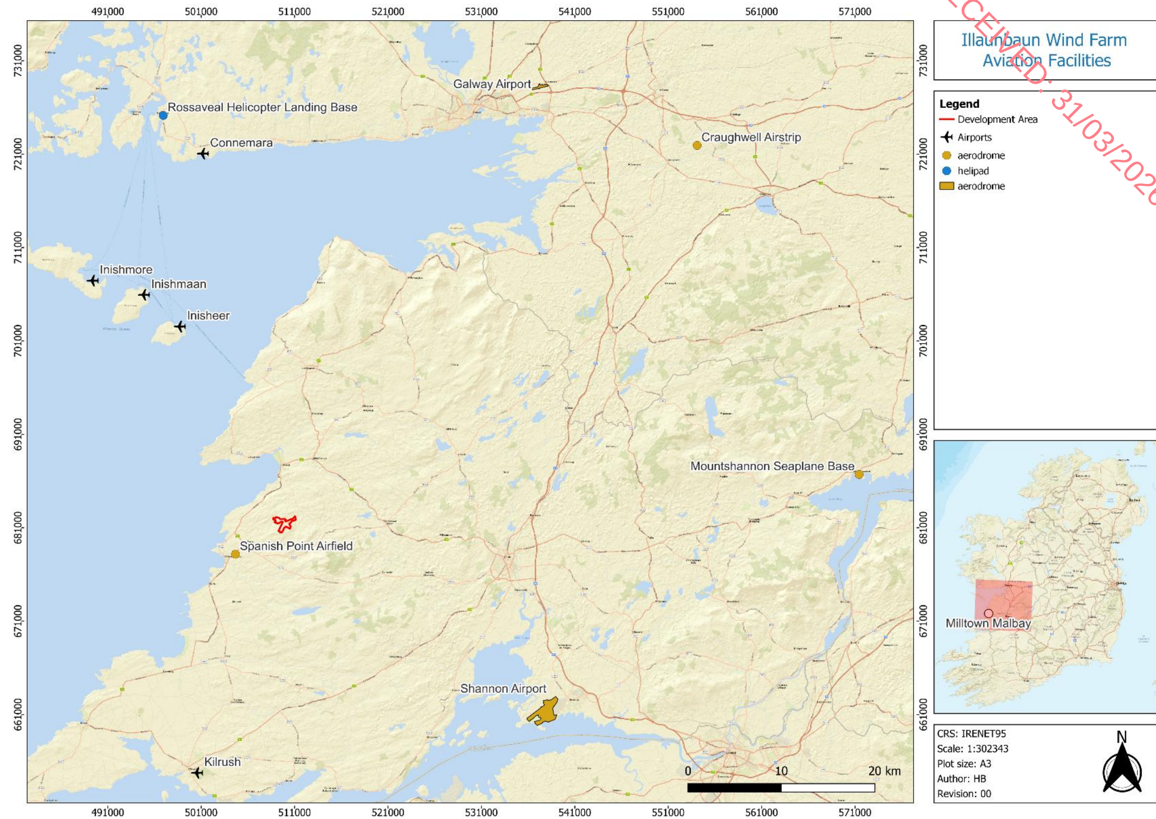
Figure 17-7: Aviation Facilities in proximity to the Proposed Development
