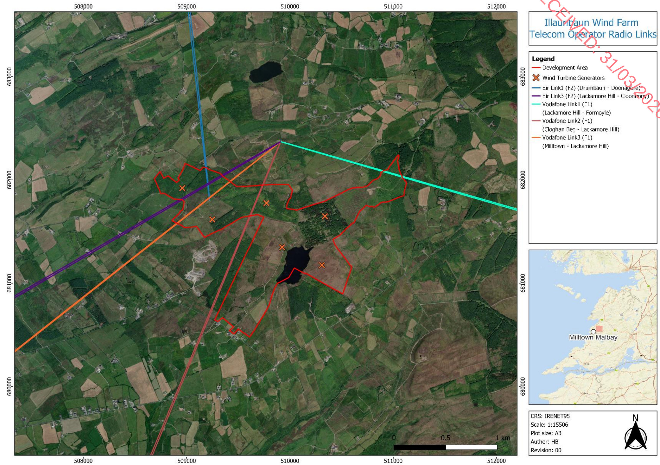
Figure 17-3: Telecommunications Operator networks shown relative to the Proposed Development
